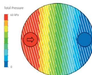
PRESSURE DISTRIBUTION
