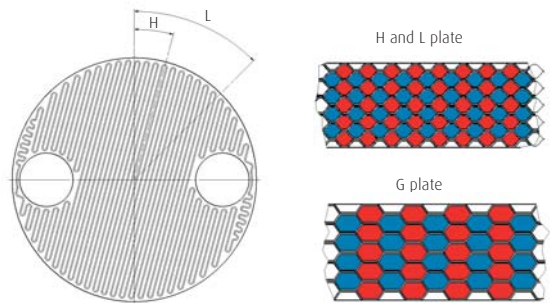
PLATE PROFILE
