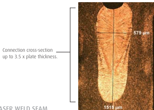
LASER WELD SEAM
